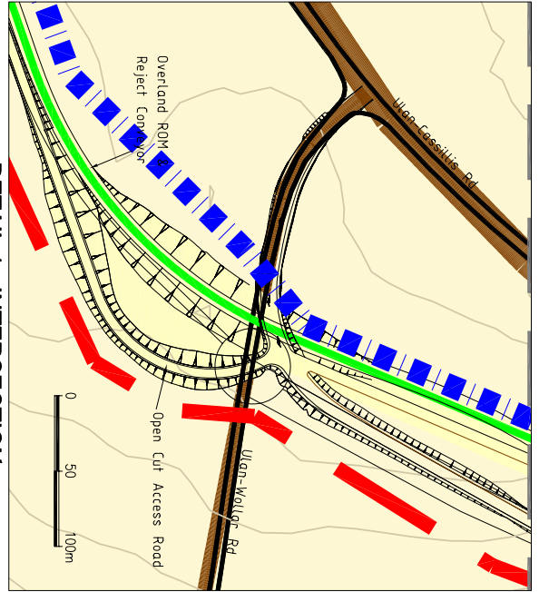
DETAIL 1 - INTERSECTION
