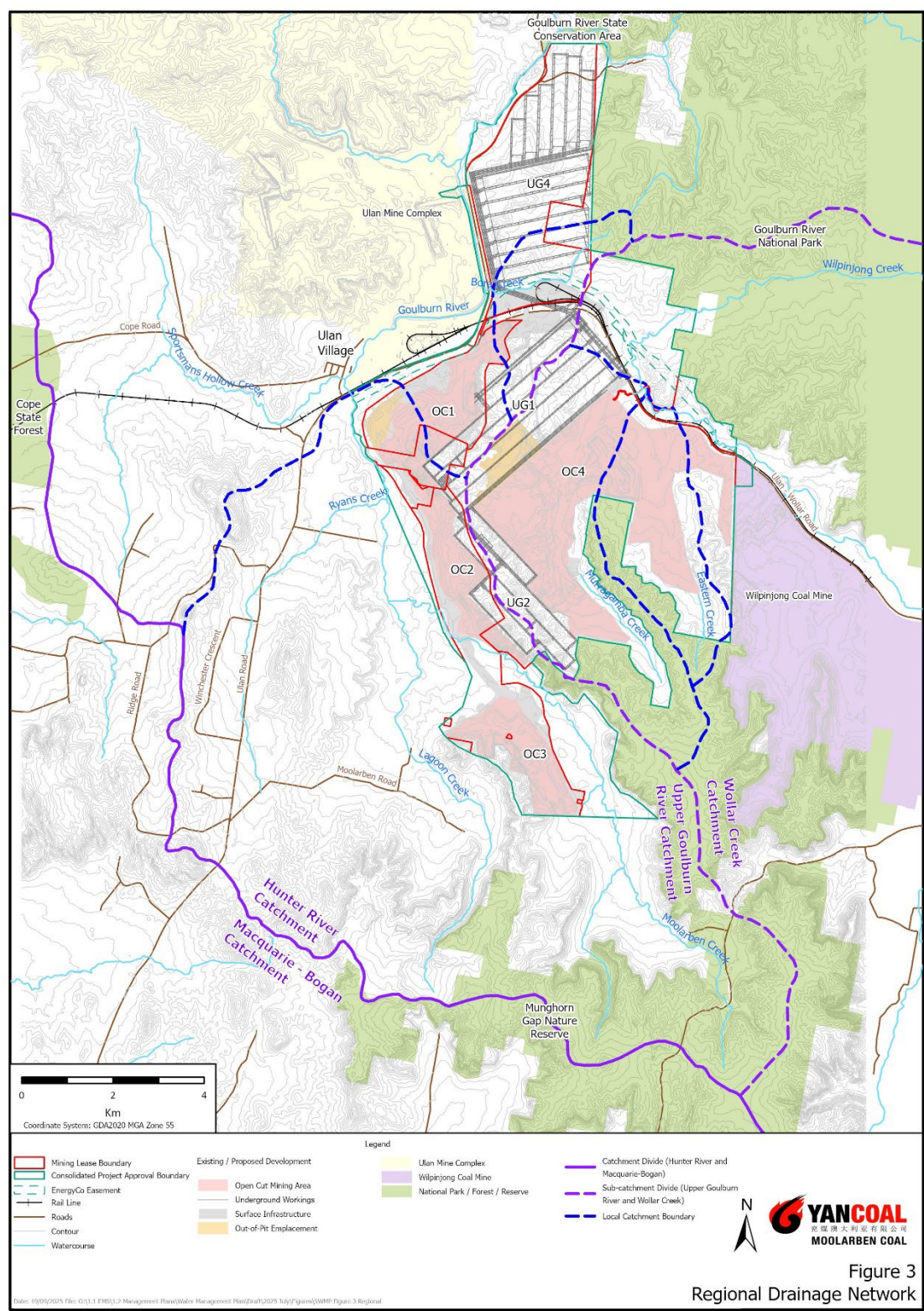
Figure 3: Regional Drainage Network
