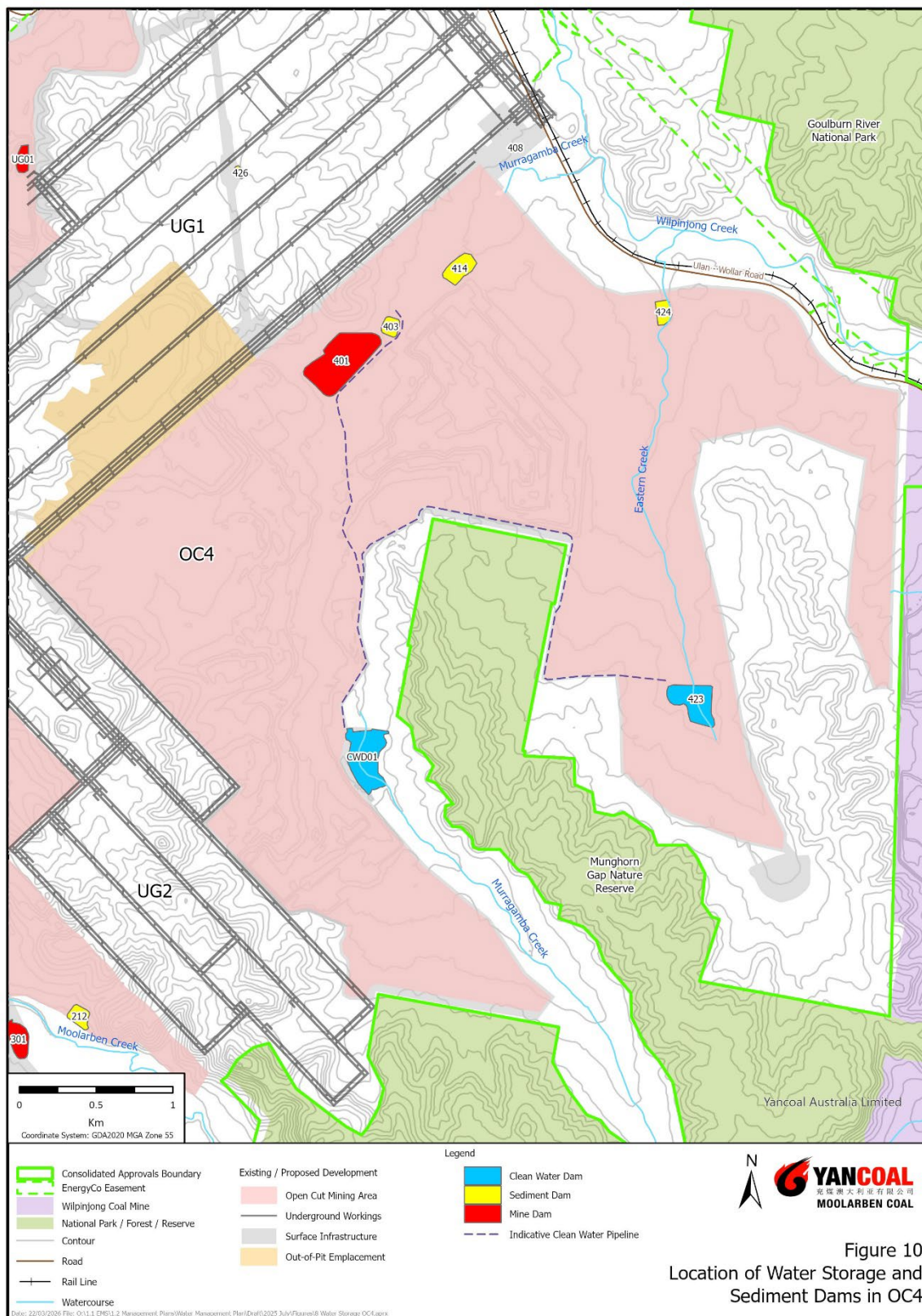
Figure 10: Location of Water Storage and Sediment Dams in OC4
