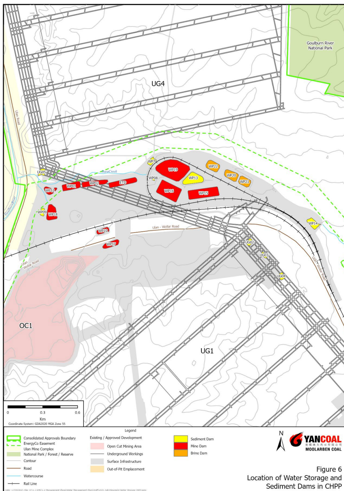
Figure 6: Location of Water Storage and Sediment Dams in CHPP Area
