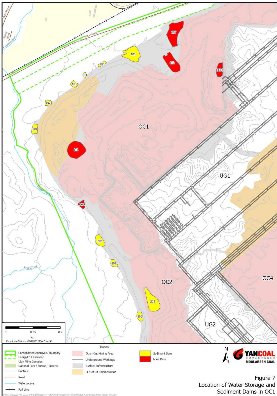
Figure 7: Location of Water Storage and Sediment Dams in OC1
