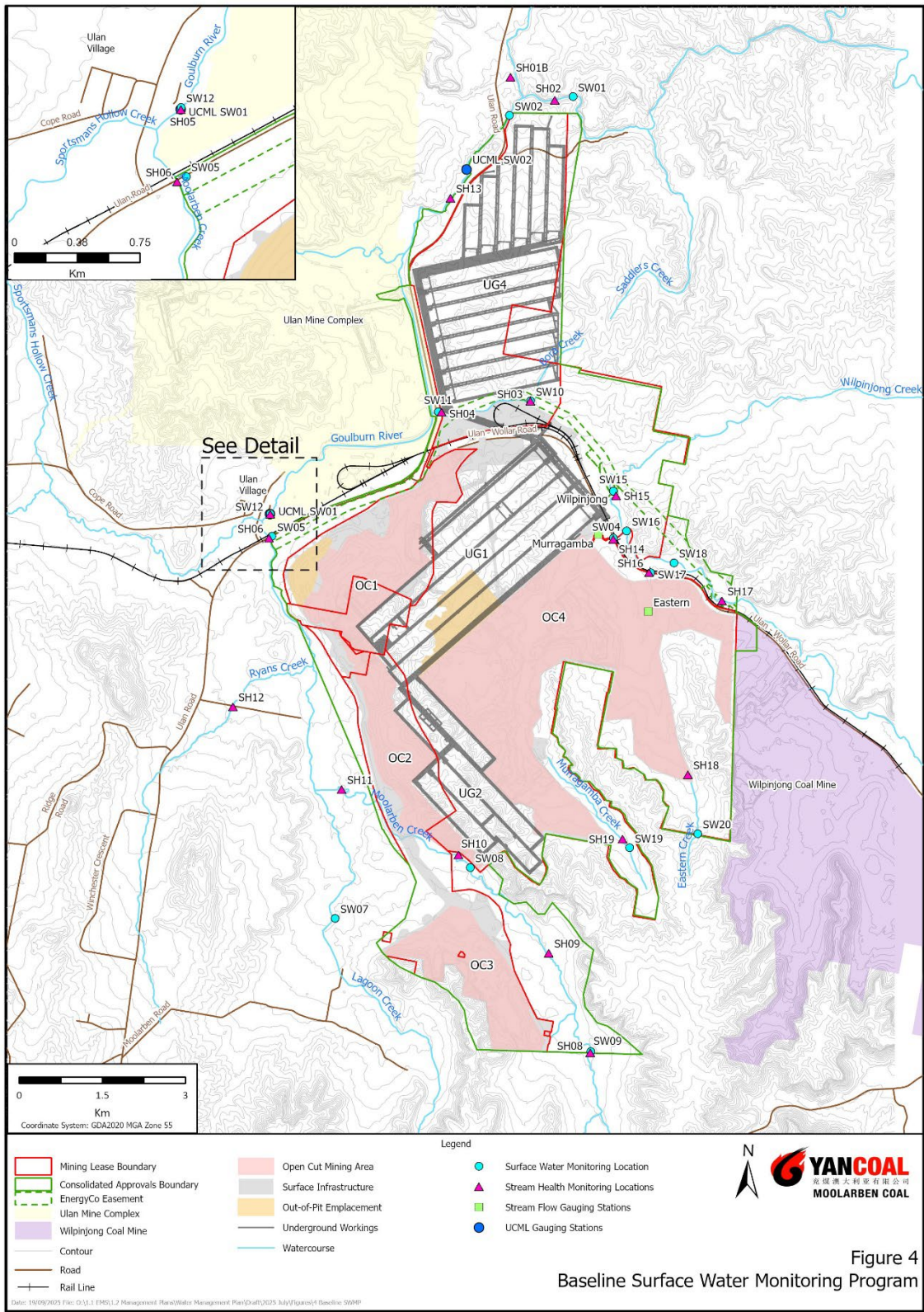
Figure 4: Baseline Surface Water Monitoring Program
