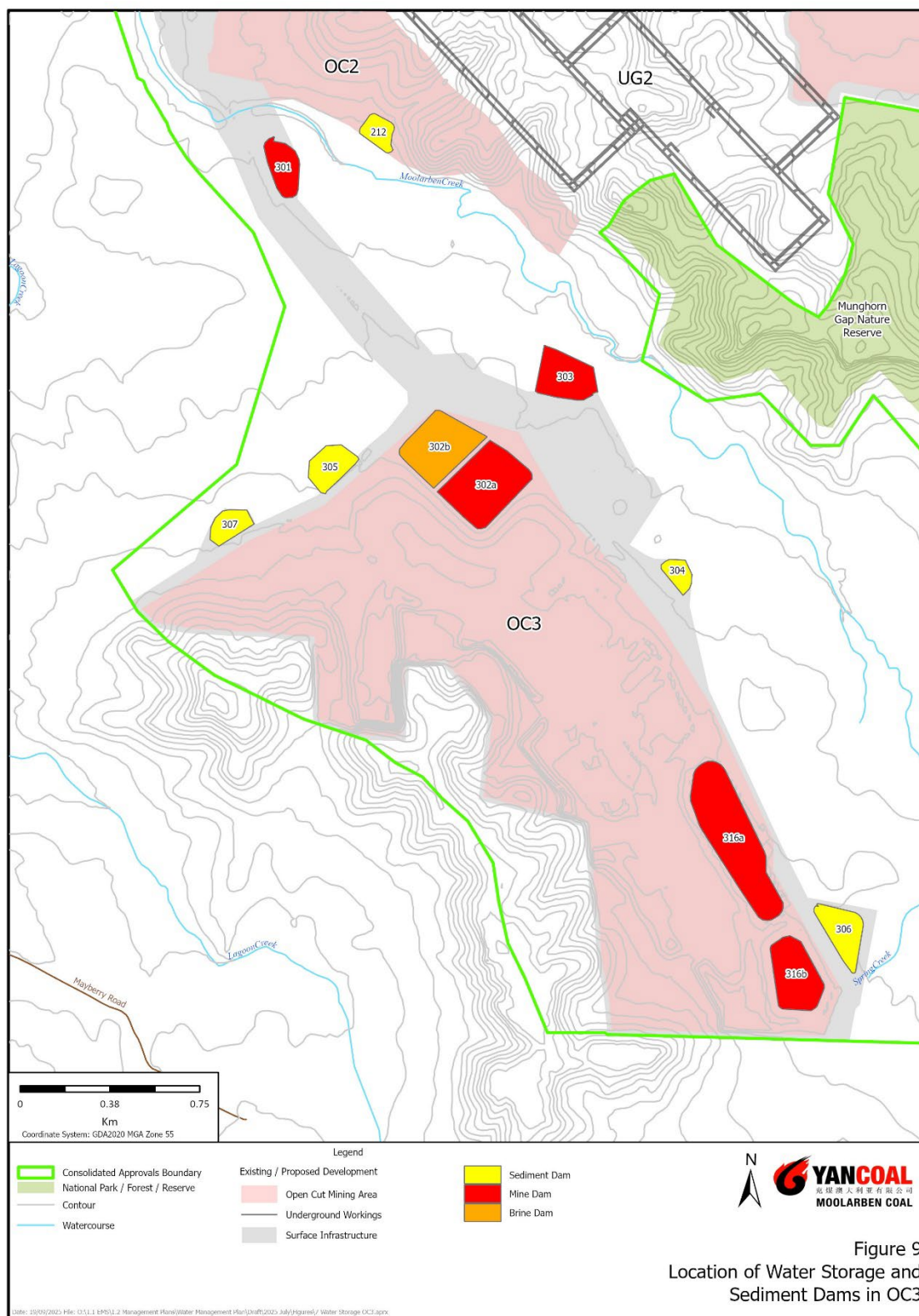
Figure 9: Location of Water Storage and Sediment Dams in OC3
