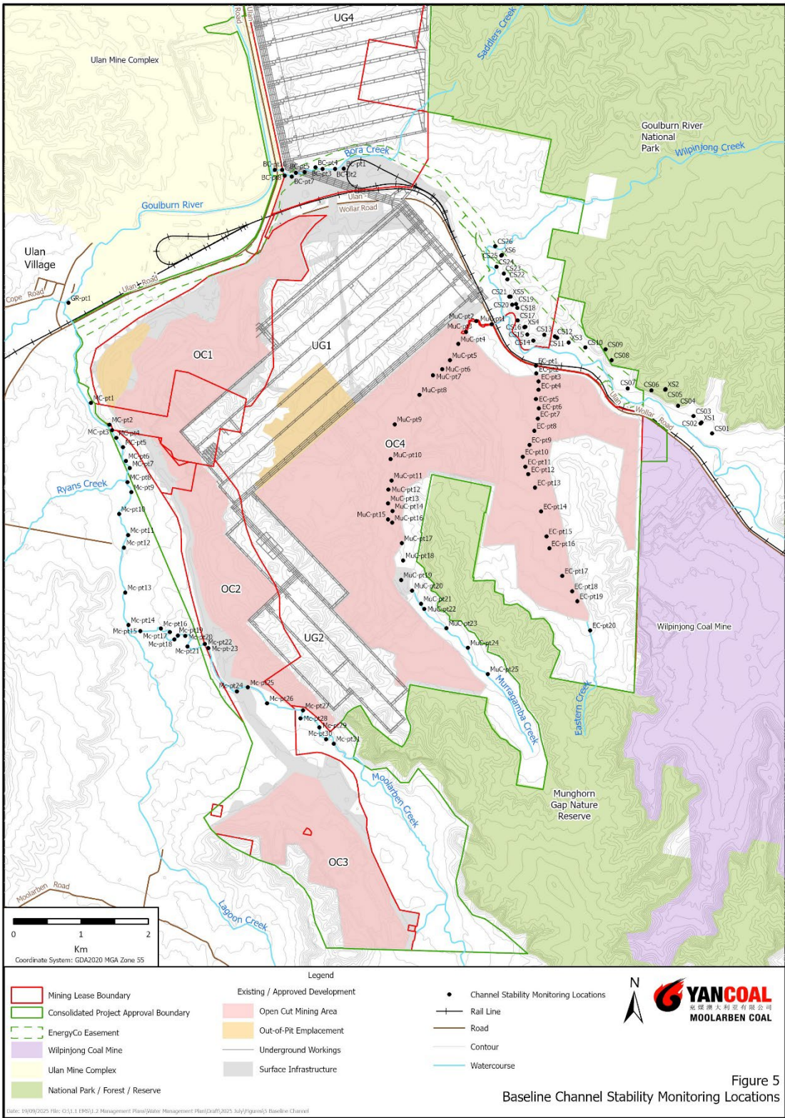
Figure 5: Baseline Channel Stability Monitoring Locations
