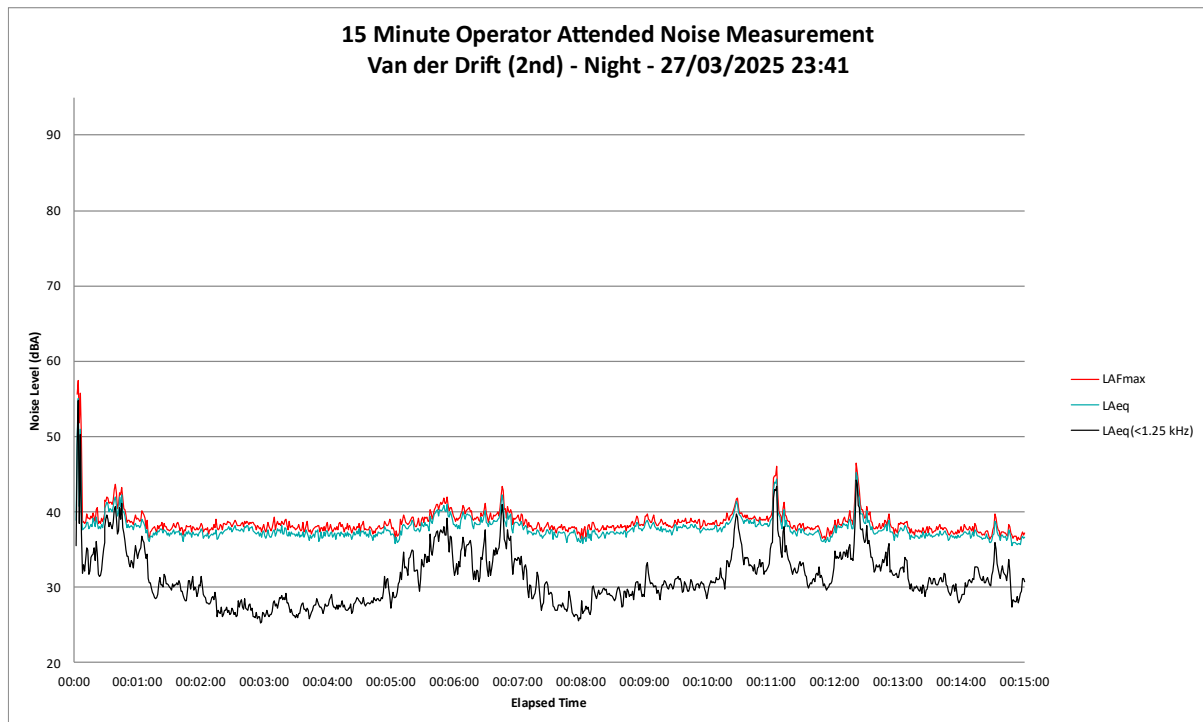
Figure B23 Night Period – ‘Van der Drift’ Secondary Operator Attended Noise Survey Results
