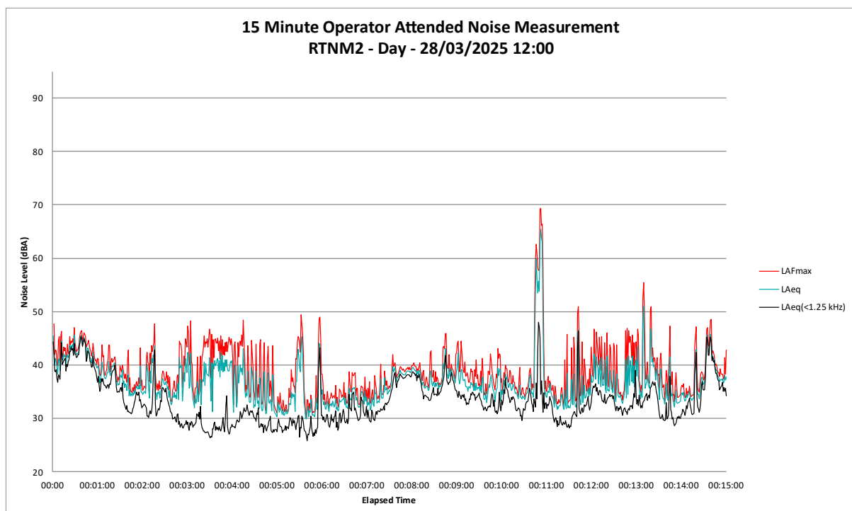
Figure B28 Day Period – ‘RTNM2 Operator Attended Noise Survey Results
