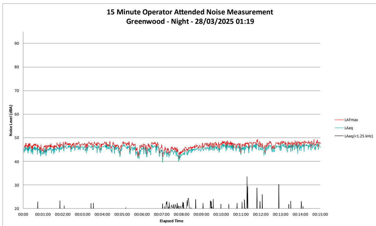
Figure B26 Night Period – ‘Greenwood’ Operator Attended Noise Survey Results
