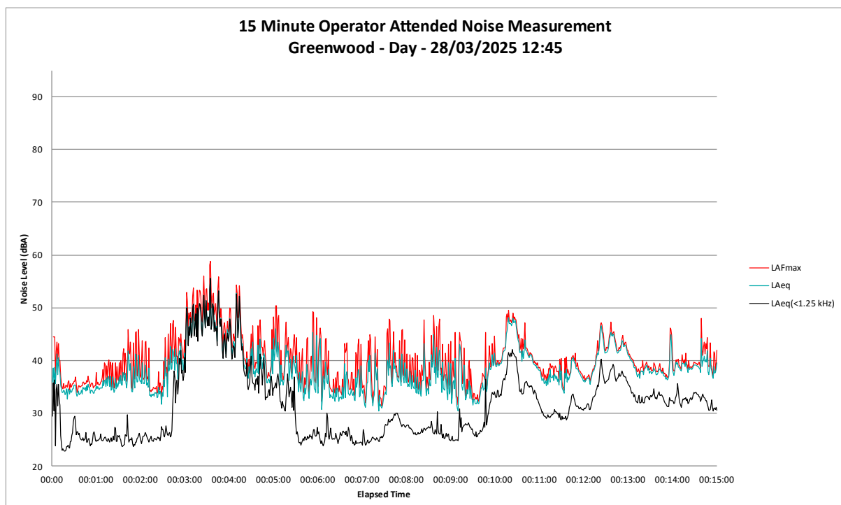
Figure B24 Day Period – ‘Greenwood’ Operator Attended Noise Survey Results
