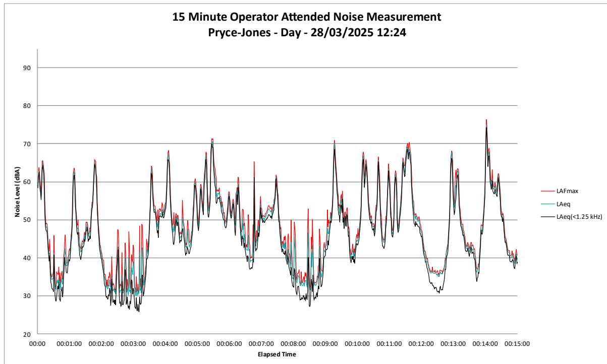
Figure B17 Day Period – ‘Pryce-Jones’ Operator Attended Noise Survey Results
