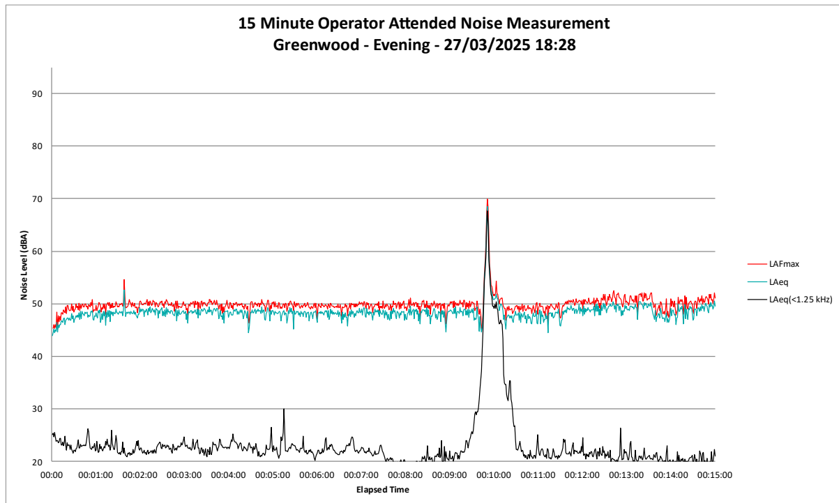
Figure B25 Evening Period – ‘Greenwood’ Operator Attended Noise Survey Results
