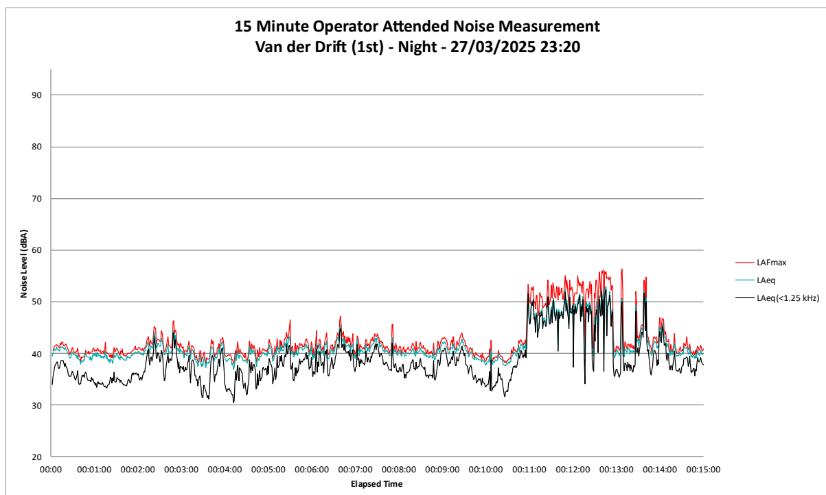
Figure B22 Night Period – ‘Van der Drift’ Operator Attended Noise Survey Results
