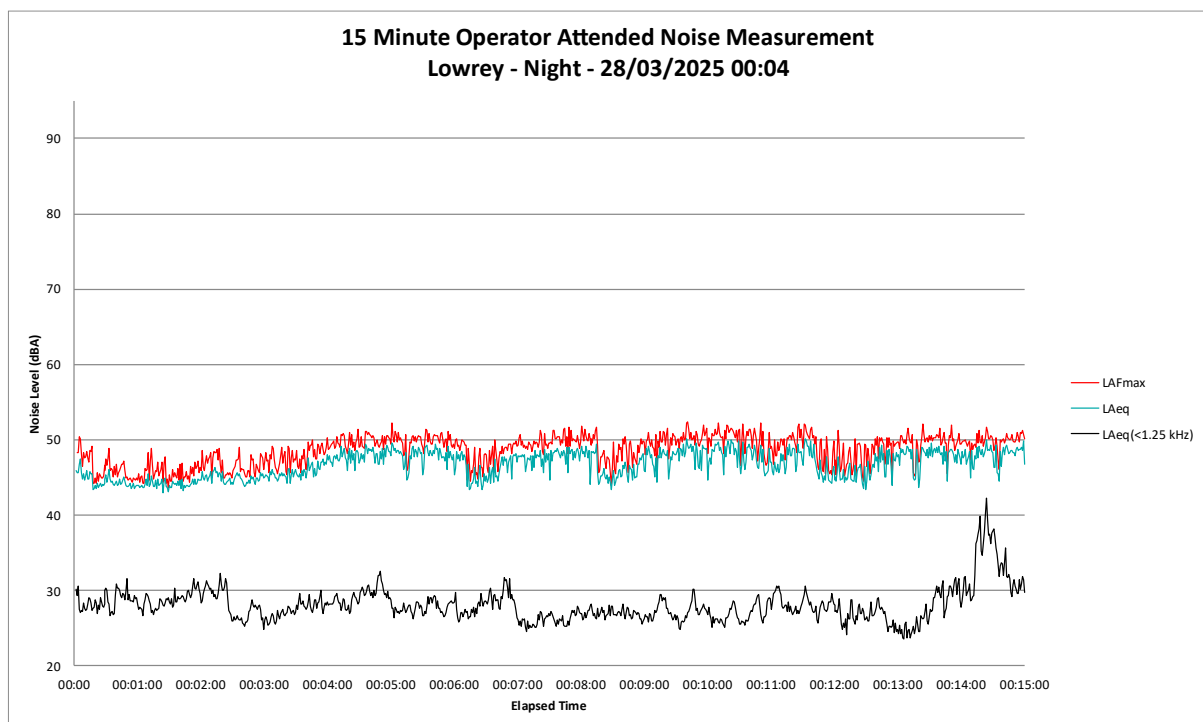
Figure B16 Night Period – ‘Lowrey’ Operator Attended Noise Survey Results
