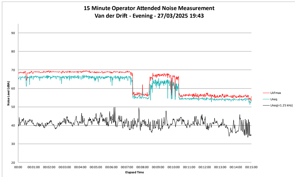
Figure B21 Evening Period – ‘Van der Drift’ Operator Attended Noise Survey Results
