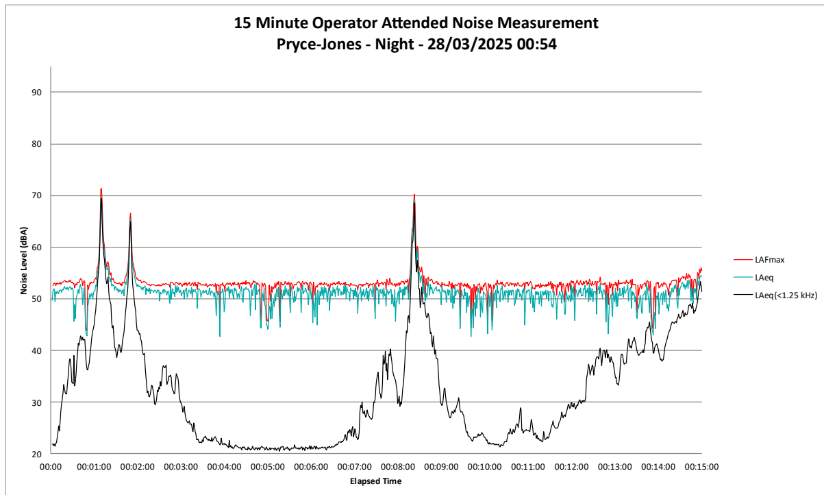
Figure B19 Night Period – ‘Pryce-Jones’ Operator Attended Noise Survey Results
