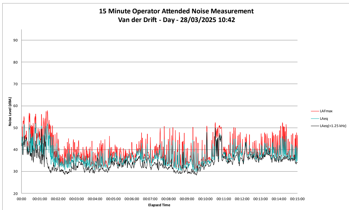
Figure B20 Day Period – ‘Van der Drift’ Operator Attended Noise Survey Results
