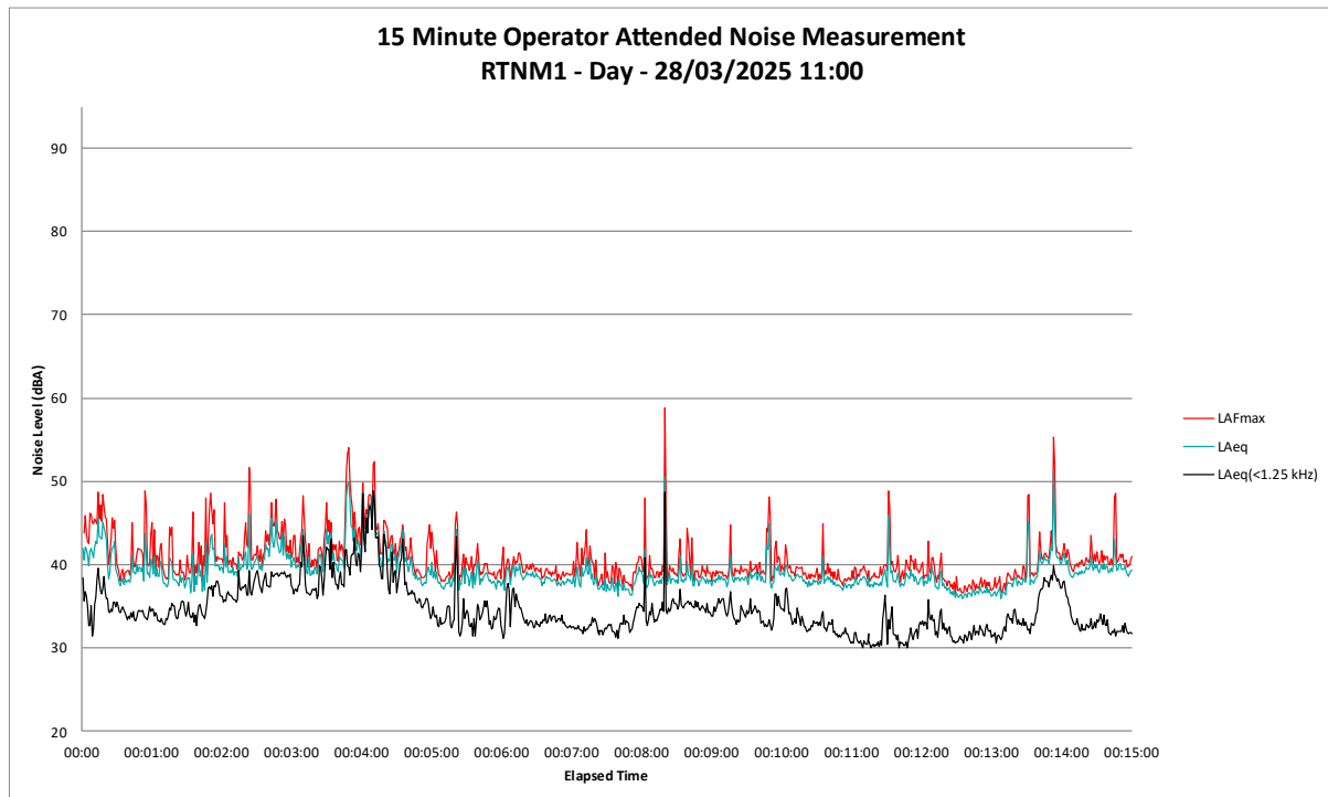
Figure B27 Day Period – ‘RTNM1 Operator Attended Noise Survey Results
