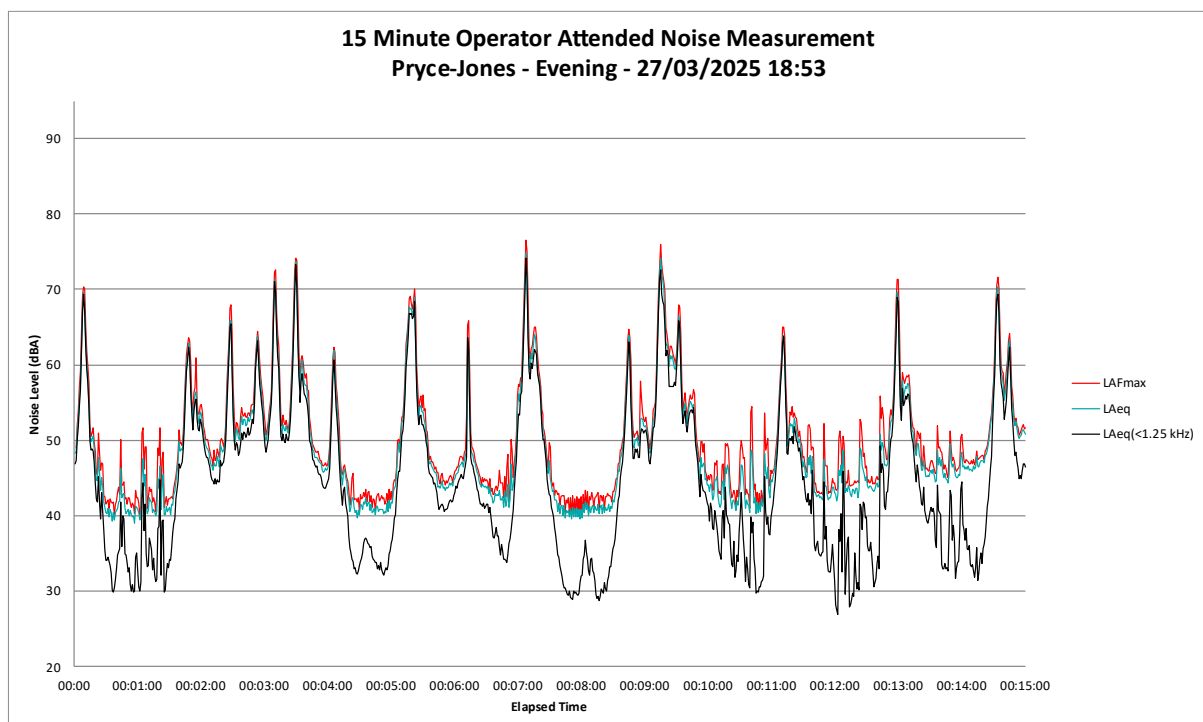
Figure B18 Evening Period – ‘Pryce-Jones’ Operator Attended Noise Survey Results
