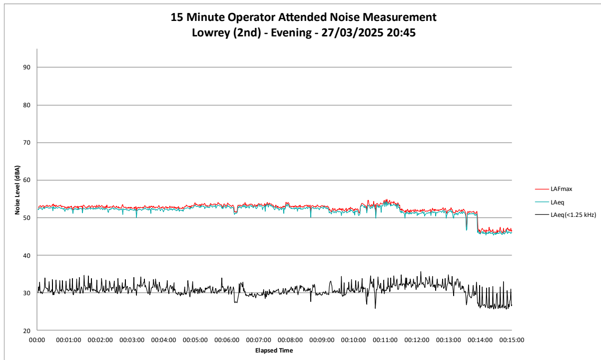
Figure B15 Evening Period – ‘Lowrey’ Secondary Operator Attended Noise Survey Results
