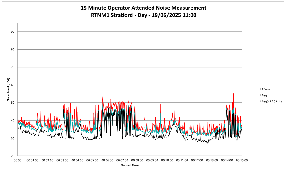
Figure B25 – Day Period – ‘RTNM1 Stratford’ Operator Attended Noise Survey Results
