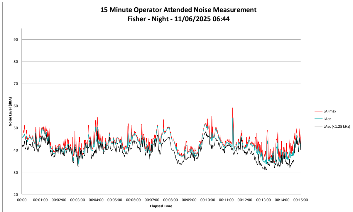
Figure B3 – Night Period – ‘NM4’ Operator Attended Noise Survey Results
